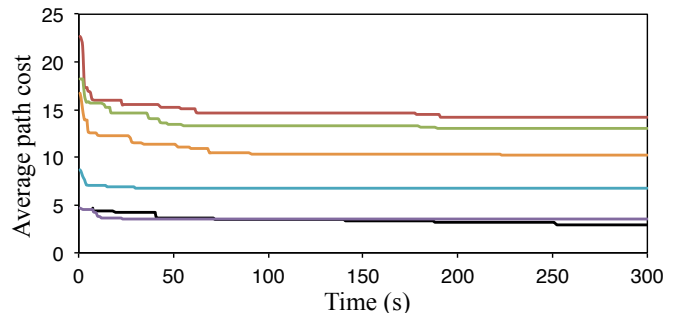
Fig. 9. Over six distinct goals (three from each lung), the cost of the best path found by time averaged over three runs each.
